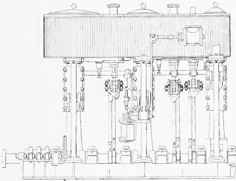
TRIPLE-EXPANSION ENGINE OF H. W. SIBLEY'S STEAM YACHT RESTLESS.—Built by F. W. Wheeler & Co., West Bay City, Mich.
